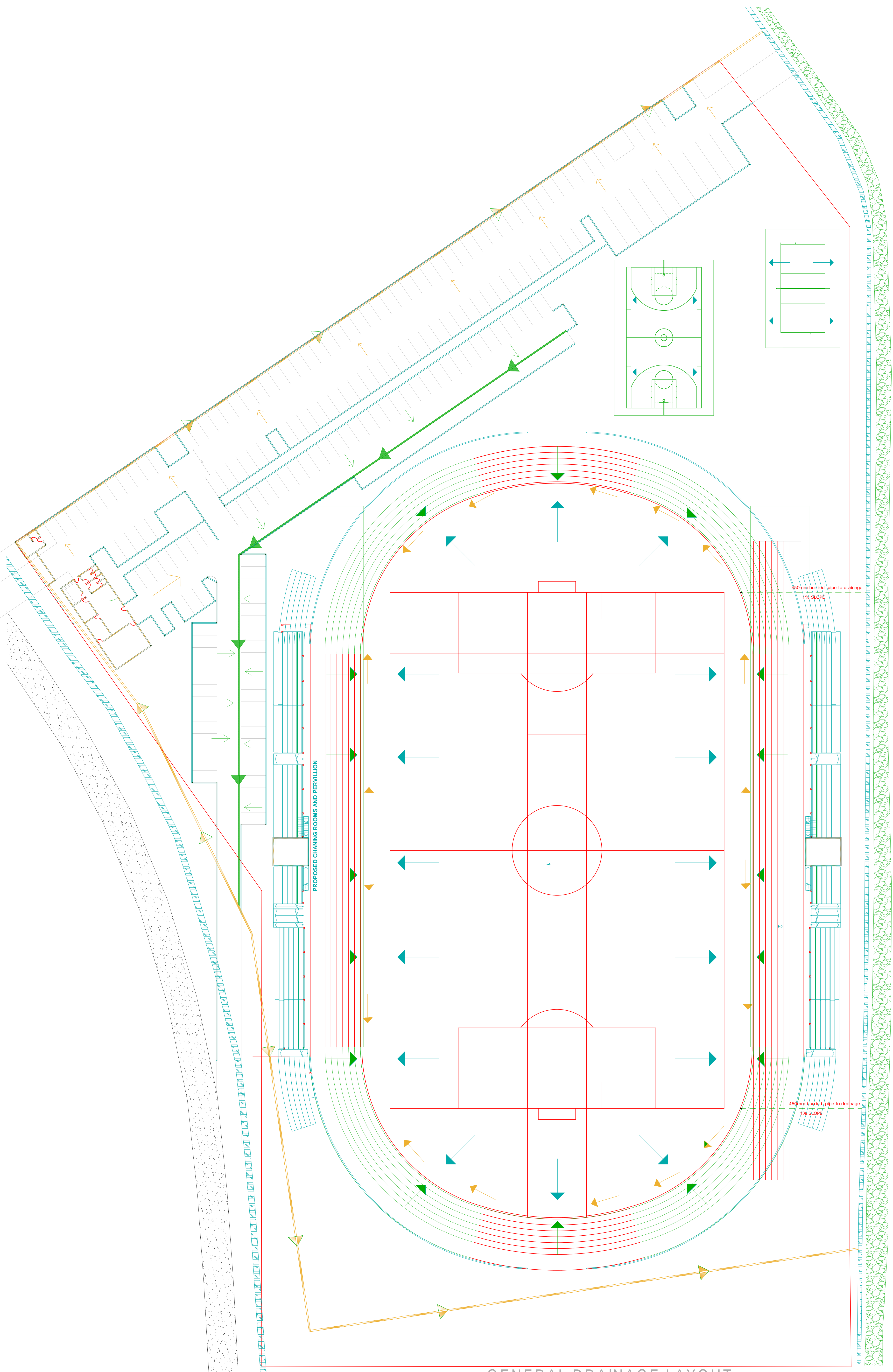
GENERAL DRAINAGE LAYOUT SCALE 1:250
