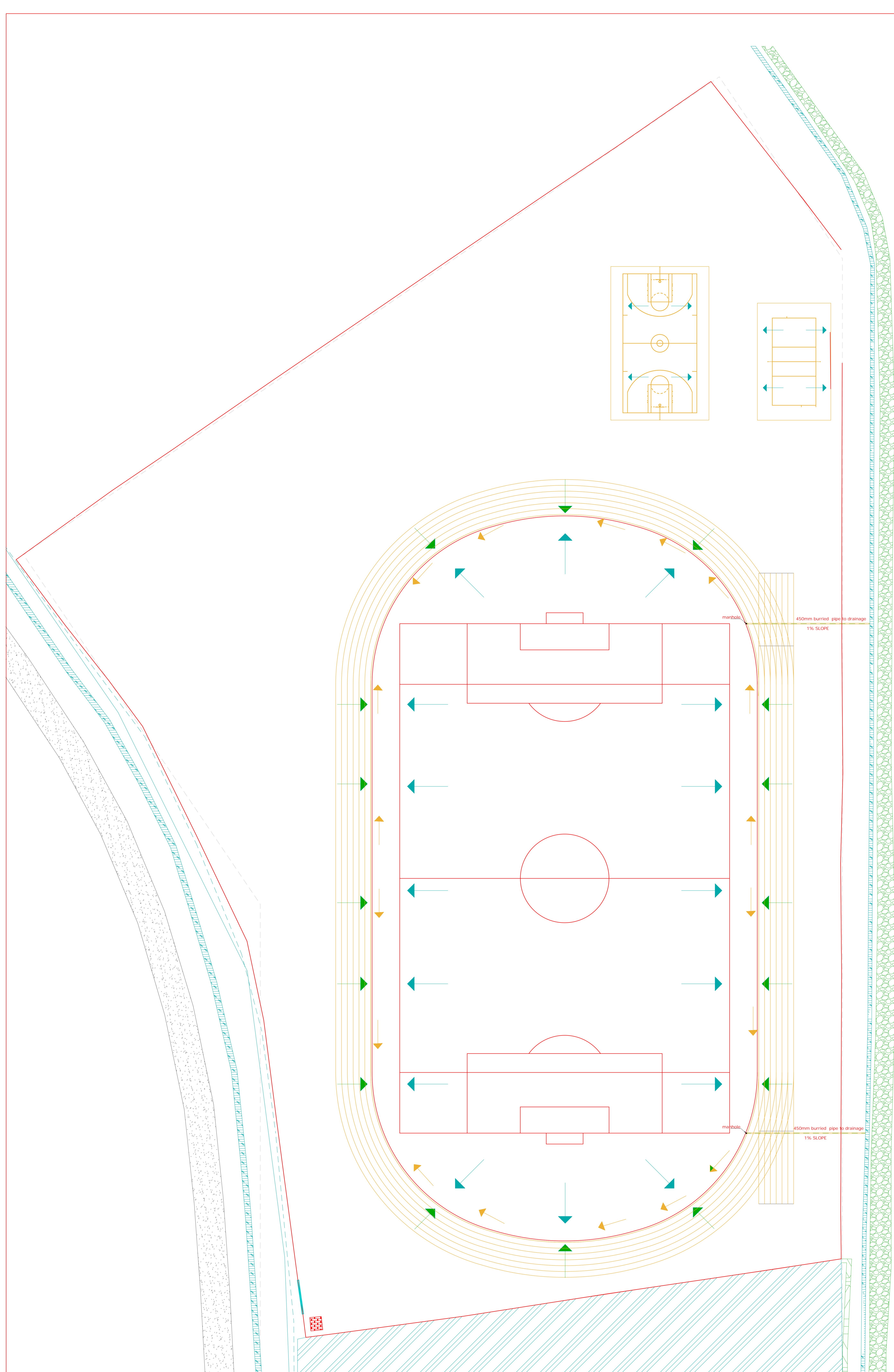
FOOTBALL,RUNNING TRACK BASKETBALL & VOLLEYBALL DRAINAGE LAYOUT SCALE 1:250
