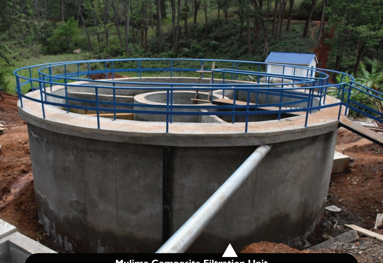
Mulima Composite Filtration Unit
